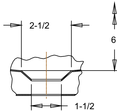
DRAIN DETAIL DETAIL A SCALE 0.350
