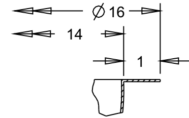
UNDER MOUNT DETAIL DETAIL C SCALE 0.375
