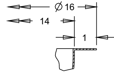
UNDER MOUNT DETAIL DETAIL C SCALE 0.375
